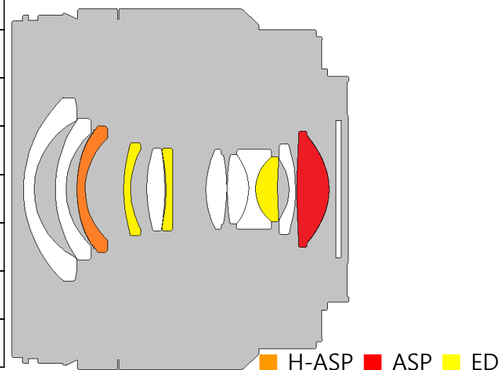
Lens Construction
